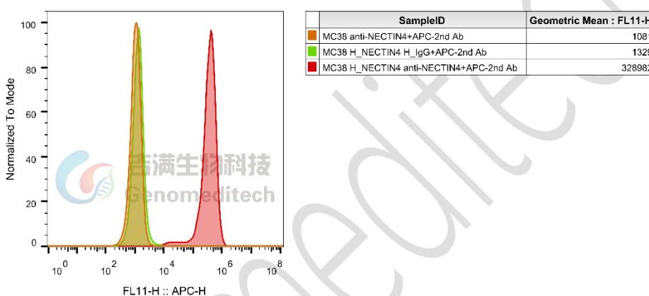
Figure 1 | H_NECTIN4 MC38 Cell Line (Cat. GM-C32901) was determined by flow cytometry using Anti-H_Nectin4 hIgG1 Antibody(Enfortumab) (Cat. GM-23369AB ).
